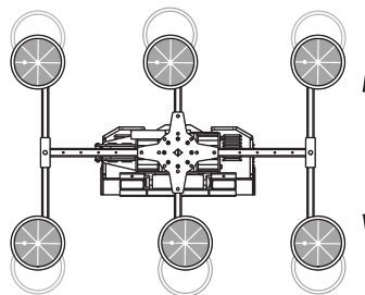
Vertical lift 300mm (12")
