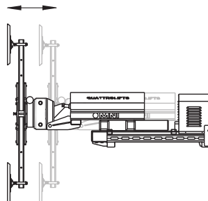
300mm (12") forward extension
